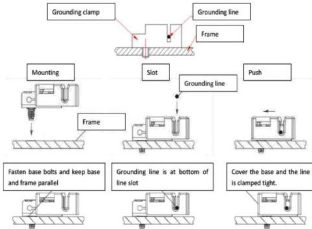
Figure 6 Grounding Clamp Installation Note: TYCO. 1954381-1 (recommended) is used in figures above
