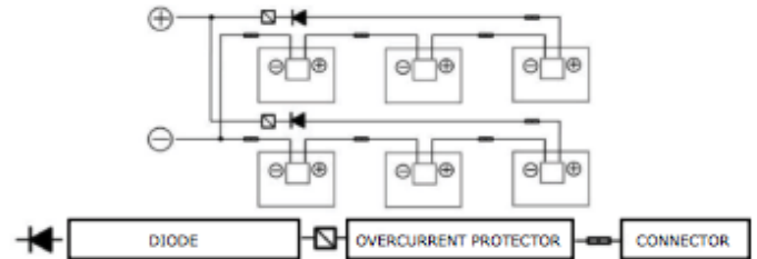
Figure 5: Series connection and parallel connection circuit diagram
